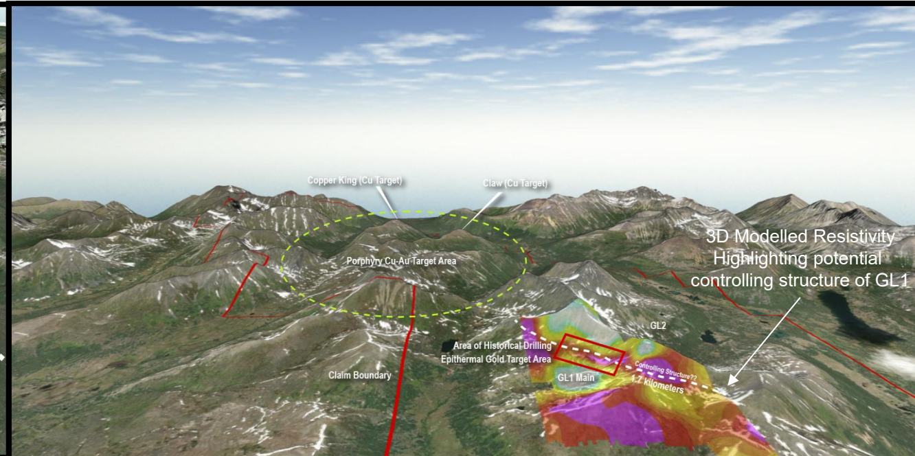
3D View of Golden Lion Property Looking North
